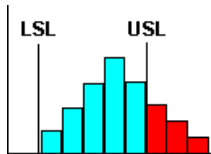
Histogram
