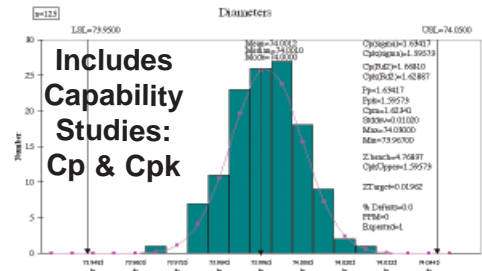
Histogram
